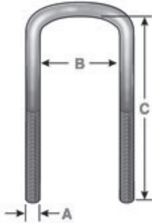
Semi-Round Bend
