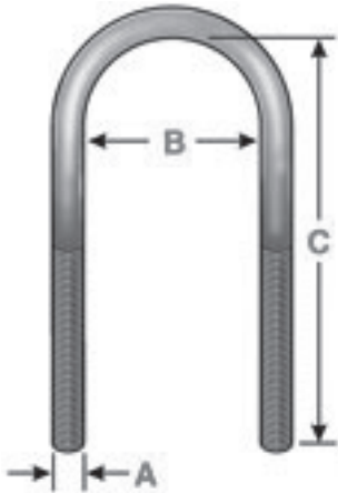
Round Bend
