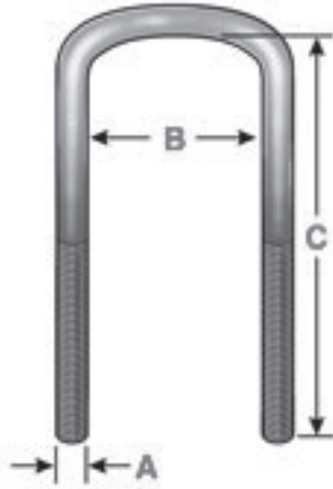
Semi-Round Bend
