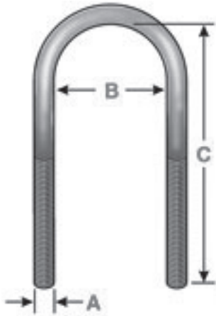
Round Bend
